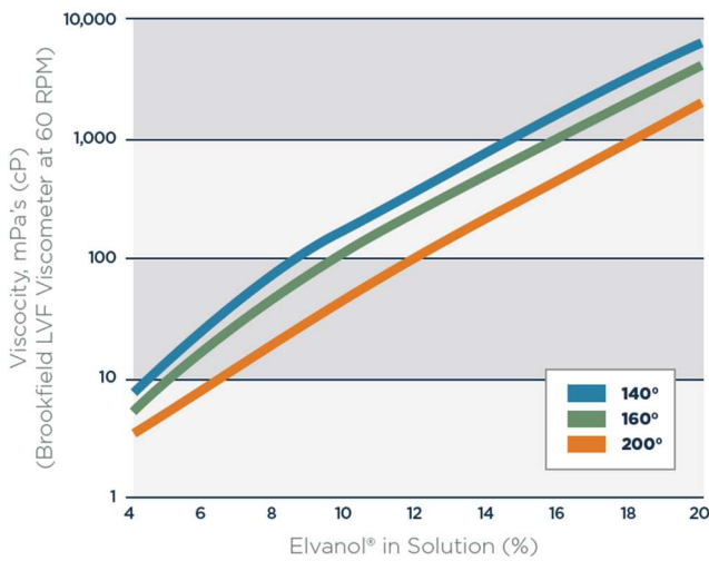
EFFECT OF CONCENTRATION AND TEMPERATURE ON VISCOSITY OF ELVANOL® T-66
